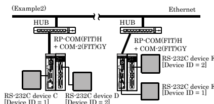
(Example2) An Ethernet cable is used to extend the connection of RS-232C device C and RS-232C device E. An Ethernet cable is used to extend the connection of RS-232C device D and RS-232C device F. (Communication is disabled between directly stacked devices.) RS-232C (device C, device ID = 1) ← Connection to Ethernet (wired LAN) → RS-232C (device E, device ID = 1) RS-232C (device D, device ID = 2) ← Connection to Ethernet (wired LAN) → RS-232C (device F, device ID = 2) * It is same when RP-COM(FIT)H-AF is replaced to RP-COM(FIT)H and when COM-1PD(FIT)GY is replaced to COM2(FIT)GY, too.
