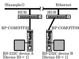
(Example1) An Ethernet cable is used to extend the connection of RS-232C device A and RS-232C device B. RS-232C (device A, device ID = 1) ← Connection to Ethernet (wired LAN) → RS-232C (device B, device ID = 1) * It is same when RP-COM(FIT)H-AF is replaced to RP-COM(FIT)H.
