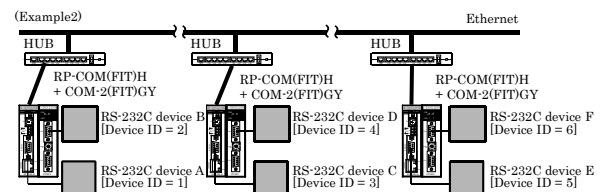
(Example2) It is possible to communicate with two or more equipment. RS-232C (device A, device ID = 1) ← Connection to Ethernet (wired LAN) → RS-232C (device C, device ID = 3) RS-232C (device A, device ID = 1) ← Connection to Ethernet (wired LAN) → RS-232C (device D, device ID = 4) RS-232C (device A, device ID = 1) ← Connection to Ethernet (wired LAN) → RS-232C (device E, device ID = 5) RS-232C (device A, device ID = 1) ← Connection to Ethernet (wired LAN) → RS-232C (device F, device ID = 6) RS-232C (device B, device ID = 2) ← Connection to Ethernet (wired LAN) → RS-232C (device C, device ID = 3) RS-232C (device B, device ID = 2) ← Connection to Ethernet (wired LAN) → RS-232C (device D, device ID = 4) RS-232C (device B, device ID = 2) ← Connection to Ethernet (wired LAN) → RS-232C (device E, device ID = 5) RS-232C (device B, device ID = 2) ← Connection to Ethernet (wired LAN) → RS-232C (device F, device ID = 6) RS-232C (device C, device ID = 3) ← Connection to Ethernet (wired LAN) → RS-232C (device E, device ID = 5) RS-232C (device C, device ID = 3) ← Connection to Ethernet (wired LAN) → RS-232C (device F, device ID = 6) RS-232C (device D, device ID = 4) ← Connection to Ethernet (wired LAN) → RS-232C (device E, device ID = 5) RS-232C (device D, device ID = 4) ← Connection to Ethernet (wired LAN) → RS-232C (device F, device ID = 6) * It is same when RP-COM(FIT)H-AF is replaced to RP-COM(FIT)H and when COM-1PD(FIT)GY is replaced to COM2(FIT)GY, too.
