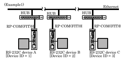
(Example1) It is possible to communicate with two or more equipment. RS-232C (device A, device ID = 1) ← Connection to Ethernet (wired LAN) → RS-232C (device B, device ID = 2) RS-232C (device A, device ID = 1) ← Connection to Ethernet (wired LAN) → RS-232C (device C, device ID = 3) * It is same when RP-COM(FIT)H-AF is replaced to RP-COM(FIT)H.
